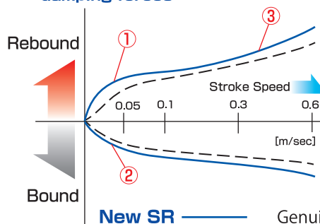
Characteristics of NewSR damping forces
